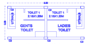
COMMON WASHROOM PLAN
