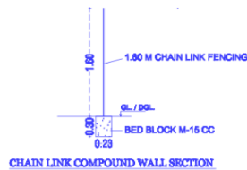
CHAIN LINK COMPOUND WALL SECTION
