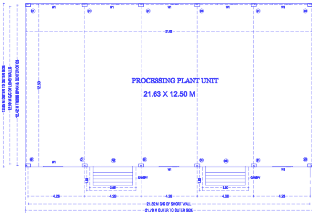
PROCESSING PLANT UNIT PLAN
